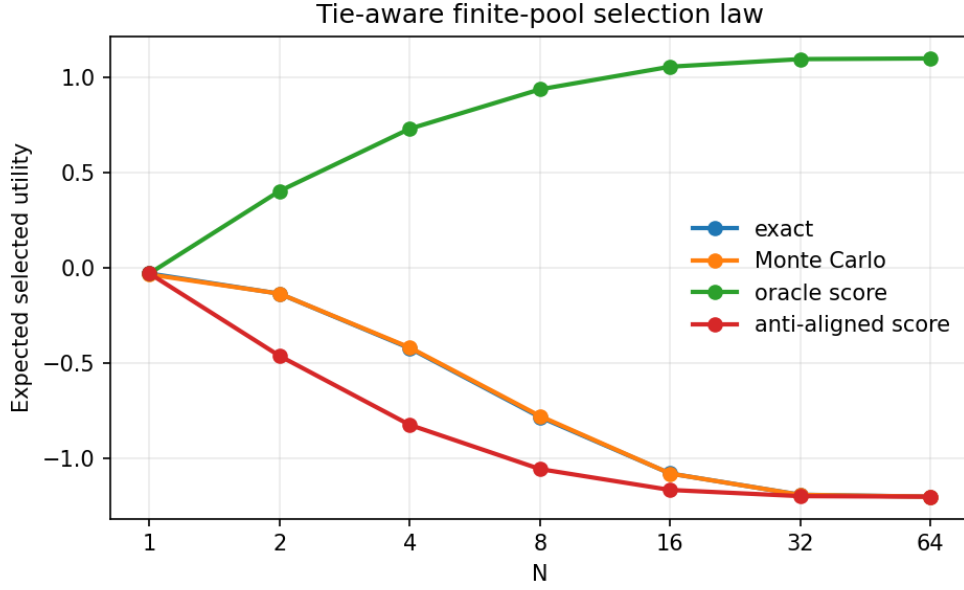
Figure 8: Tie-aware finite-law validation. Exact selected utility and Monte Carlo estimates agree within 0.0057 maximum absolute error.
